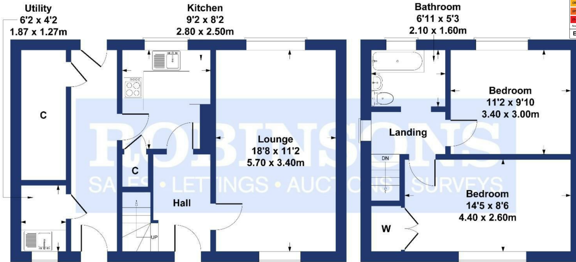
GROUND FLOOR
